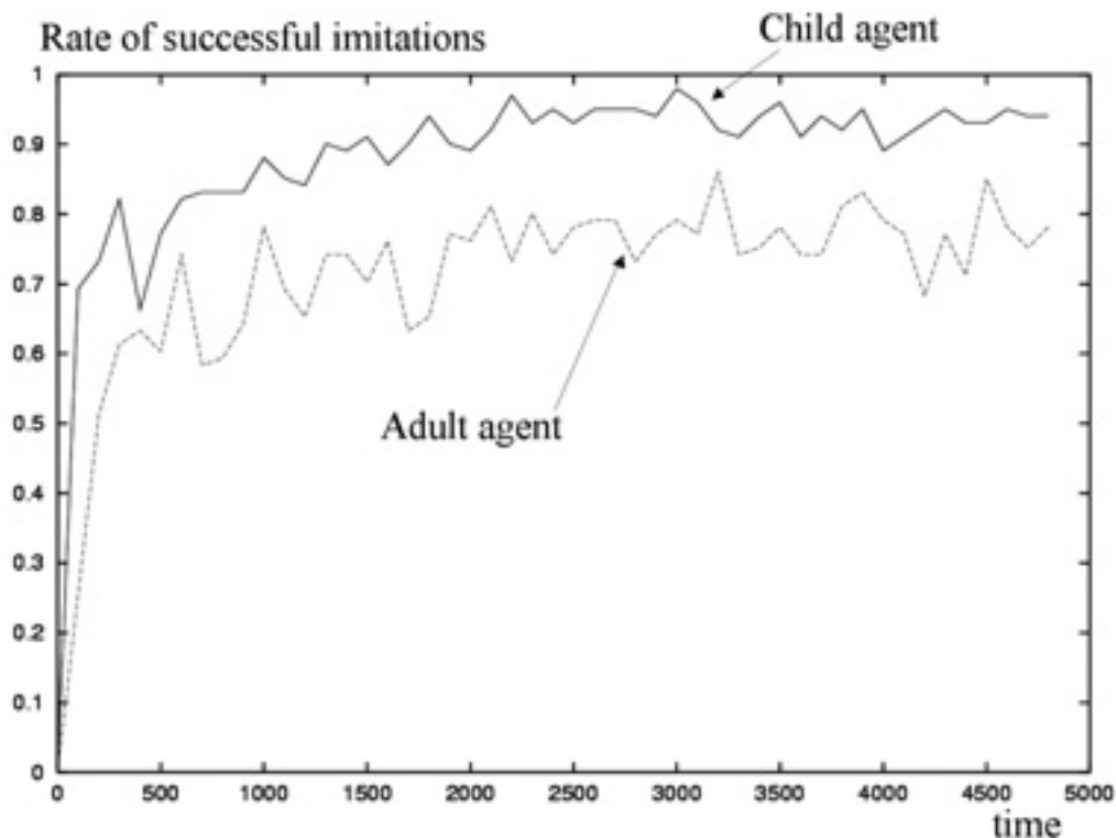
Figure 3 Evolution of the rate of successful imitations for a child agent which learns an already established syllable system (top curve), and for an adult agent already knowing another established syllable system (bottom curve). We observe that the child learns the syllable system very well, while the adult never manages to master it. This shows the "second language learning effect": adults are no longer capable of perfectly learning a new vocalization system.
