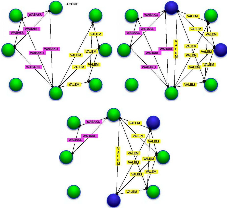
Fig. 11. Agents network dynamics. Top left: a link between two agents (i.e., nodes) exists every time they have a word in common in their inventories, so that multiple links are allowed. In this representation, a word corresponds to a fully connected (sub) set of agents, i.e., a clique; the two cliques corresponding to words WABAKU and VALEM are highlighted. Top right: the two highlighted agents have just failed to communicate, so that the word VALEM has been transmitted to the agent placed on top of the graphical representation. It therefore enters into the enlarged clique corresponding to the transmitted word VALEM. Bottom: the two highlighted agents have just succeeded using word VALEM. The clique corresponding to the used word does not change in any respect, but the competing cliques (here that of WABAKU) are reduced.
