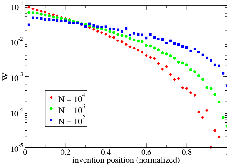
Fig. 18. Role of the system size on the distribution of the winning word. The advantage of early invention increases in larger populations.
