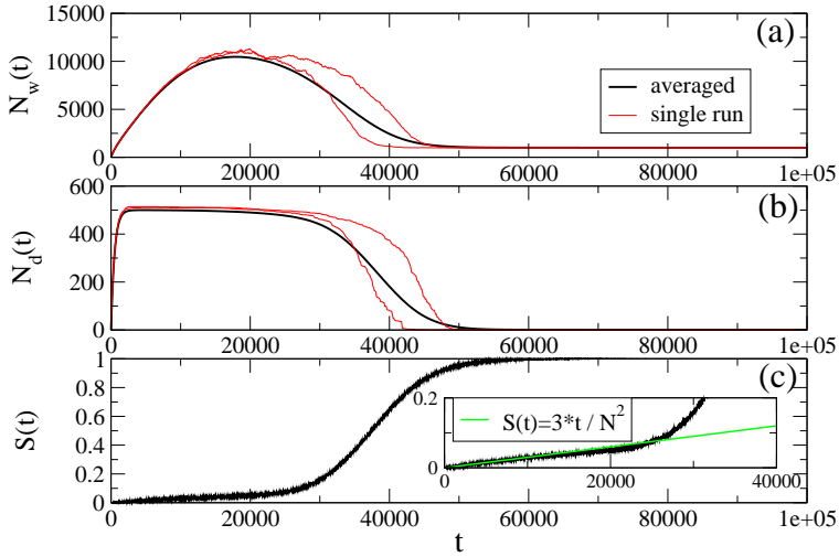
Fig. 2. Basic global quantities. (a) Total number of names present in the system, N_w(t) ; (b) Number of different names, N_d(t) ; (c) Success rate S(t) , i.e., probability of observing a successful interaction at a time t . The inset shows the linear behavior of S(t) at small times. All curves concern a population of N = 10^3 agents. The system reaches the final absorbing state, described by N_w(t) = N , N_d(t) = 1 , and S(t) = 1 , in which a global agreement on the form (name) to assign to the meaning (individual object) has been reached.
