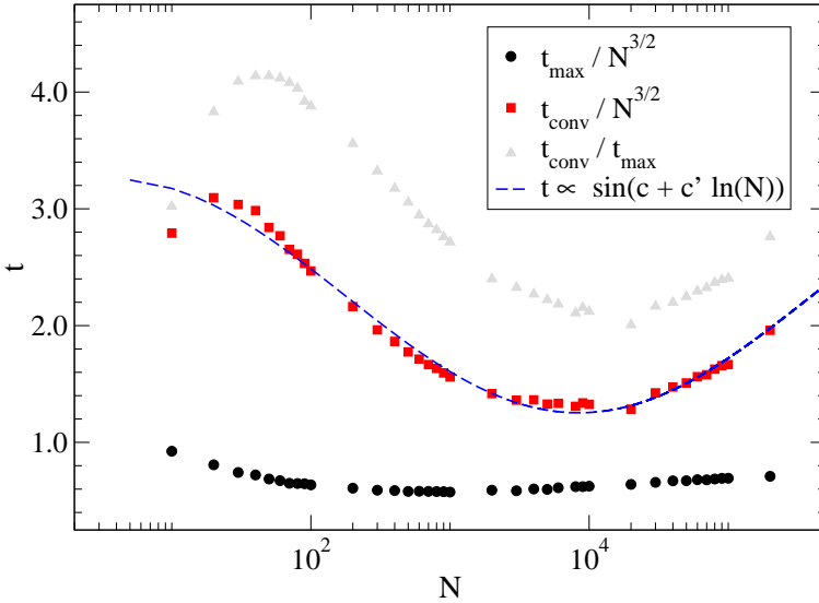
Fig. 5. Log-periodic oscillations for convergence times. Rescaled values of t_{\text{conv}} and t_{\text{max}} are plotted along with their ratio. The rescaled convergence times exhibit global oscillations that are well fitted by the function t \propto \sin(c + c' \ln(N)) , where c and c' are constants whose values are c \approx 1.0 and c' \approx 0.4 .
