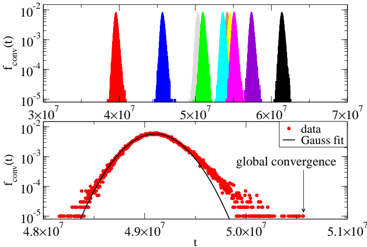
Fig. 14. Single agent convergence time distribution. We define the convergence time of a single agent the last time in which it had to delete words after successful interactions; f_{\text{conv}}(t) is the fraction of agents who reach convergence at time t . Top: distributions coming from 10 simulation runs are plotted. It is clear that distributions coming from different runs can be non-overlapping, i.e., that the distance between the peaks of single curves can be much larger than the average width of the same curves (that does not exhibit any strong dependence on the single run). Bottom: a single distribution is analyzed, showing that it cannot be described by a Gauss distribution. The last agent to converge determines the global convergence time. Curves are relative to a population of N = 10^5 agents.
