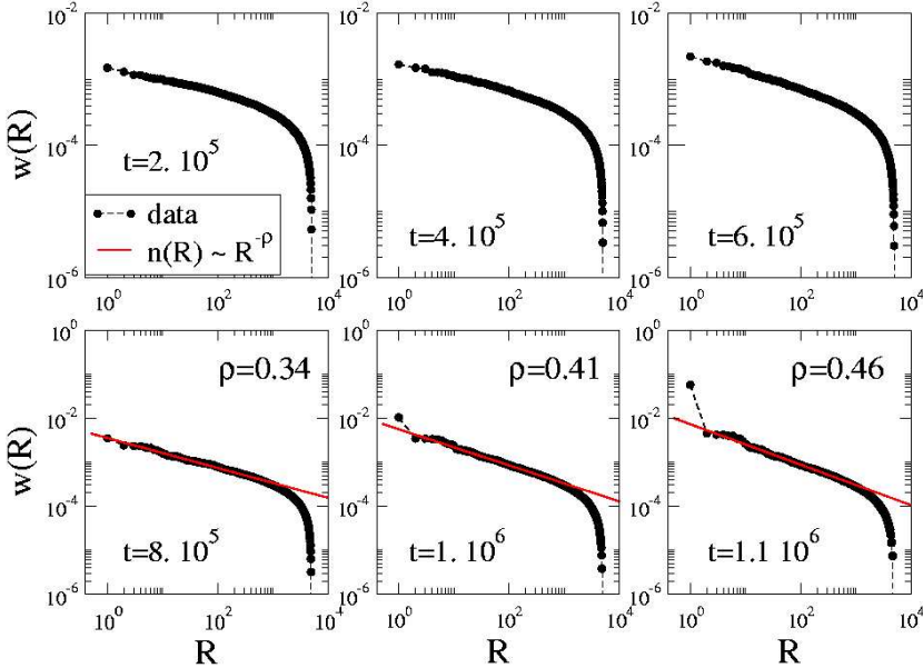
Fig. 10. Distribution w(R) of words of rank R . The most popular word has rank R = 1 , the second R = 2 , etc. The distribution follows a power-law behavior w(R) \sim R^{-\rho} with an exponent that varies in time, while for high ranks it is truncated at R \approx N/2 . Close to the disorder-order transition, however, the most diffused word abandons the distribution that keeps describing the less popular words. Data come from a single simulation run and concern a population of N = 10^4 agents.
