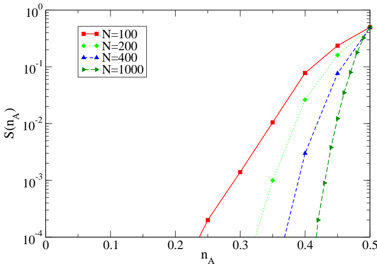
Fig. 19. Resistance against invasion. Two populations that converged separately on conventions A and B merge. The probability S(n_A) that convention A becomes the final accepted convention of the new population, versus the normalized size n_A (where n_A + n_B = 1 ) of the original population of A spreaders is plotted. As the total population size increases, the probability for the initially less diffused convention to impose itself decreases, as predicted by Eq. (14).
