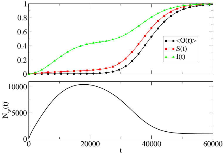
Fig. 12. Overlap functional O(t) . Top: the evolution in time of the overlap functional averaged on 1000 simulation runs (for a population of N = 10^3 agents). Curves for the success rate, S(t) , and the average intersection between inventories, I(t) , are also included. By definition, O(t) \leq 1 . It is evident that it holds \langle O(t + 1) \rangle > \langle O(t) \rangle , which, along with the stronger \langle O(t + 1) \rangle > O(t) valid for almost all configurations (not shown), indicate that the system will reach the final state of convergence, where O(t) = 1 . Bottom: The total number of words N_w(t) is plotted for reference.
