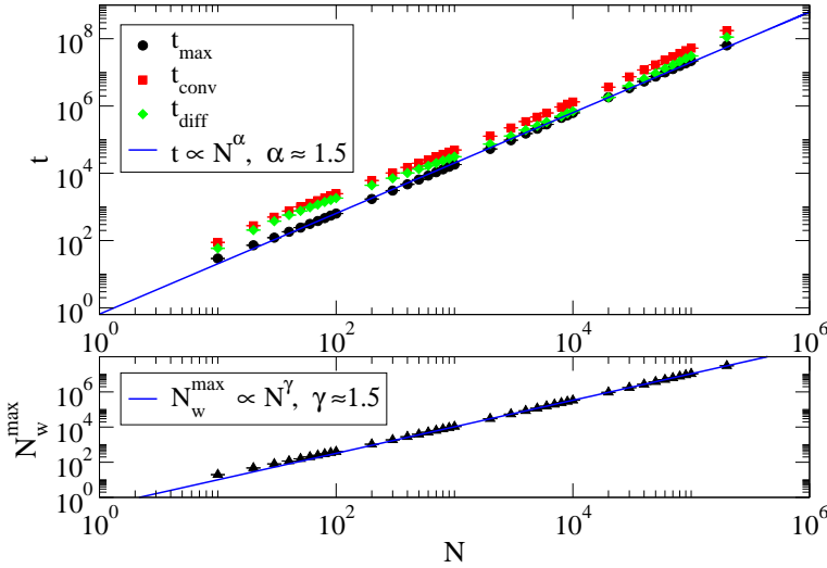
Fig. 3. Scaling with the population size N . In the upper graph the scaling of the peak and convergence time, t_{\max} and t_{\text{conv}} , is reported, along with their difference, t_{\text{diff}} . All curves scale with the power-law N^{1.5} . Note that t_{\text{conv}} and t_{\text{diff}} scaling curves present characteristic log-periodic oscillations (see Sec. 3.2). The lower curve shows that the maximum number of words (peak height, N_w^{\max} = N_w(t_{\max}) ) obeys the same power-law scaling.
